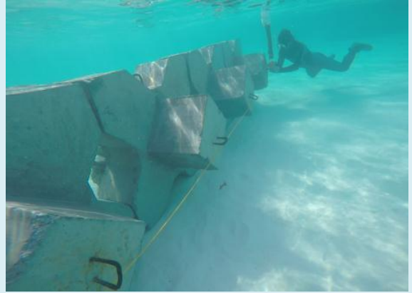
Pamalican Resorts, Inc. Underwater Installation of X-Blocks at Cuyo , Palawan
